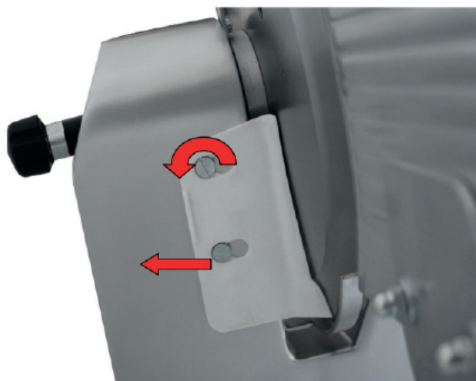
Removing the knife cover and knife squeegee
